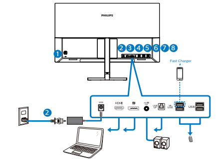
USB hub
